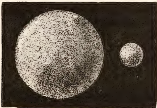
258. Comparative Dimensions of the Earth and Moon.
